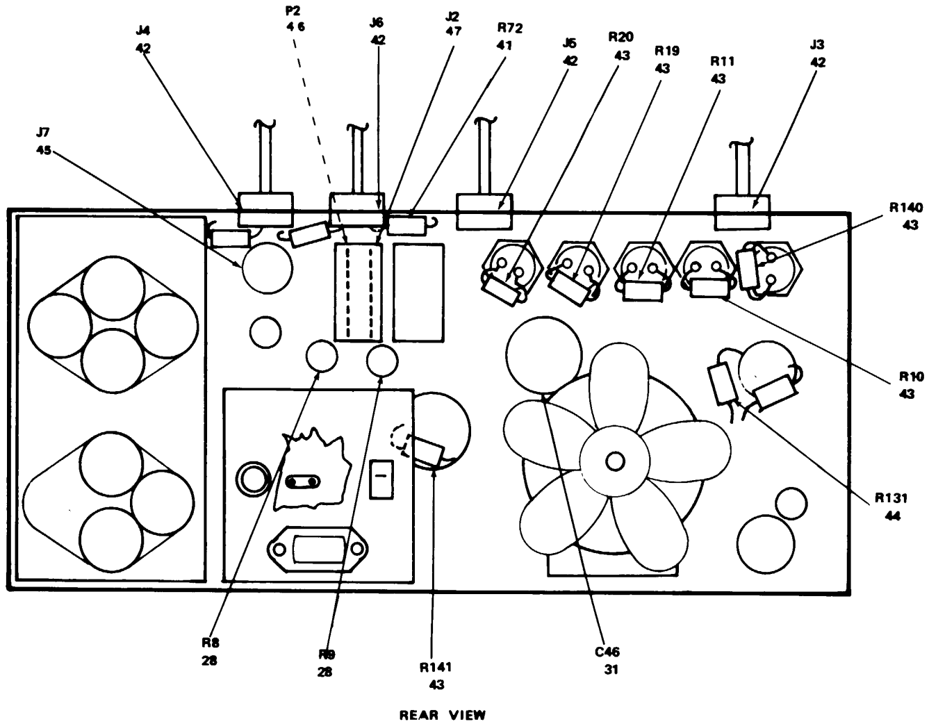
Figure 1. Signal Generator AN/USM-48 (HP628A) (Sheet 4 of 5).
