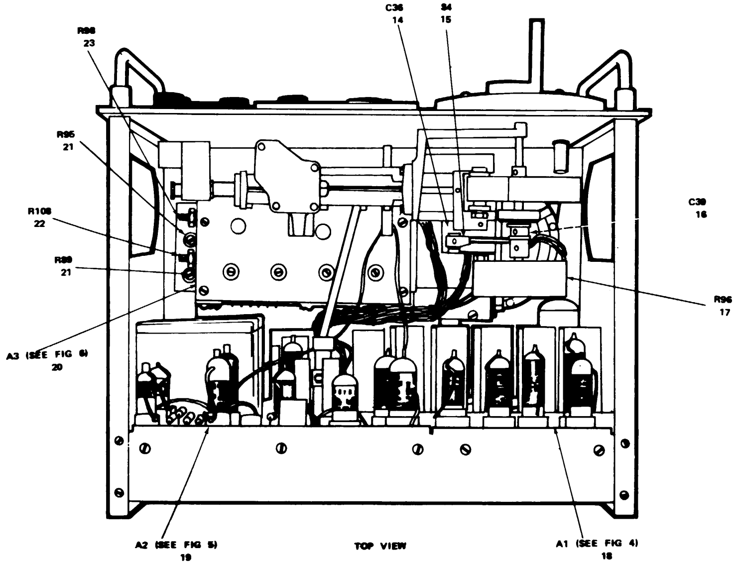
Figure 1. Signal Generator AN/USM-48 (HP628A) (Sheet 2 of 5).
