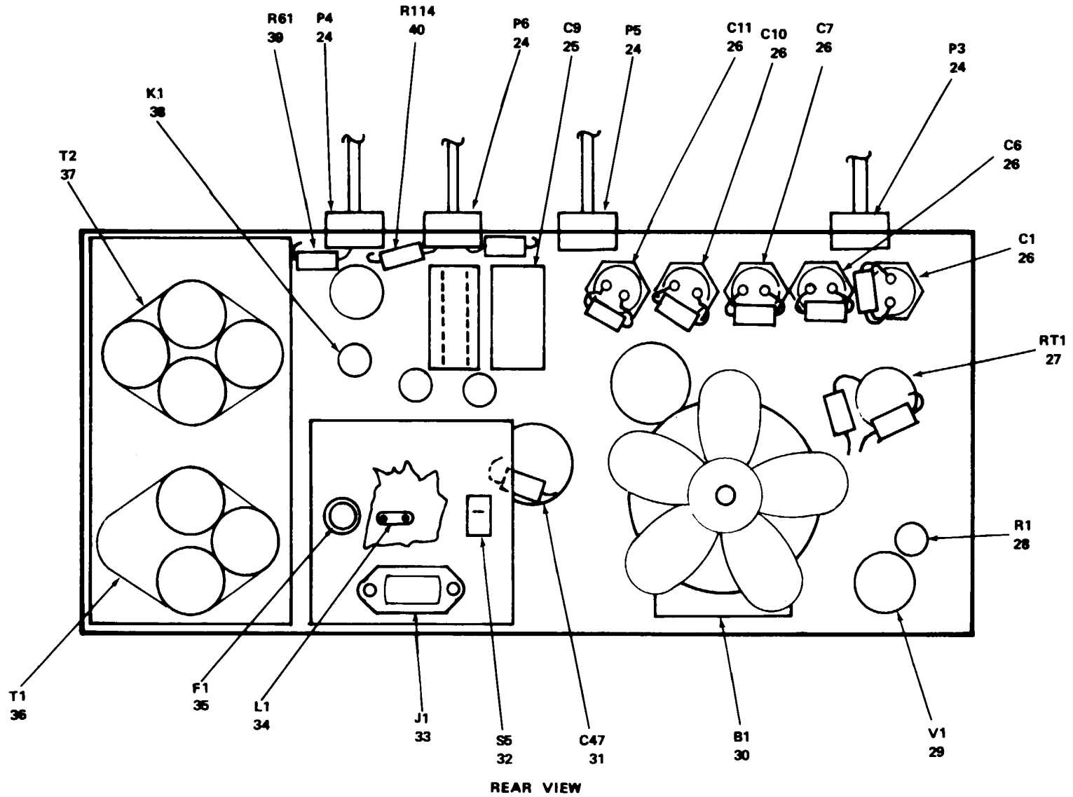
Figure 1. Signal Generator AN/USM-48 (HP628A) Sheet 3 of 5).
