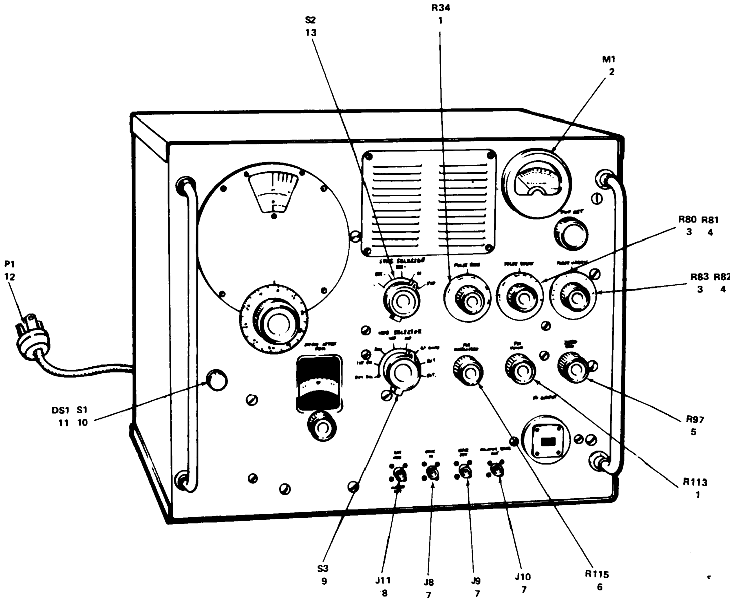
Figure 1. Signal Generator AN/USM-48 (HP628A) (Sheet 1 of 5).
